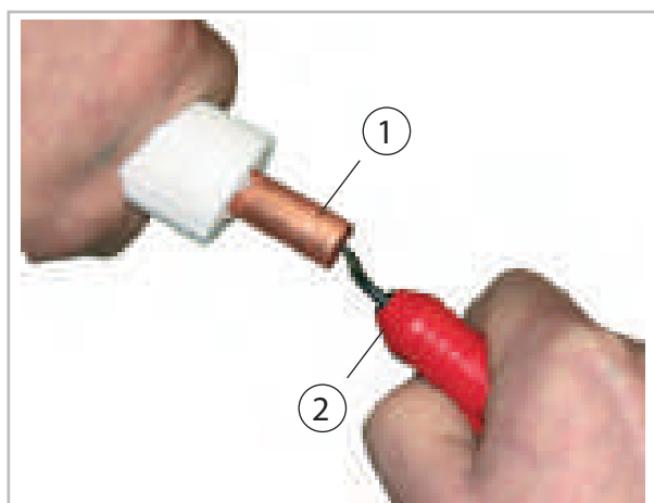
Fig. 52: Deburring the refrigerant piping
