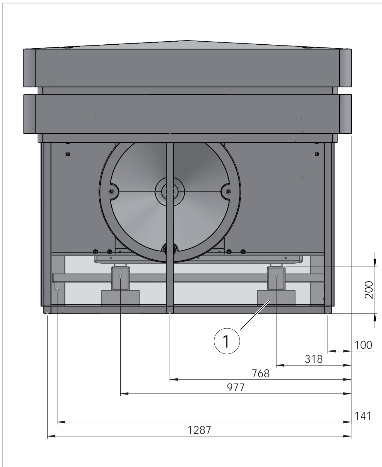
Fig. 2: Front view noise protection hood SWK 4 (all dimensions in mm)
