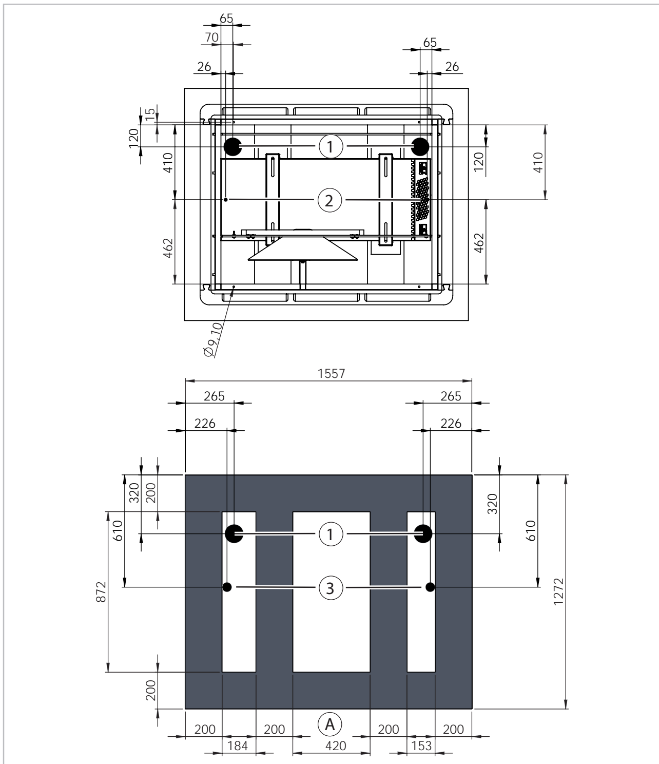
Fig. 9: Strip foundation SWK 5 and SWK 7
