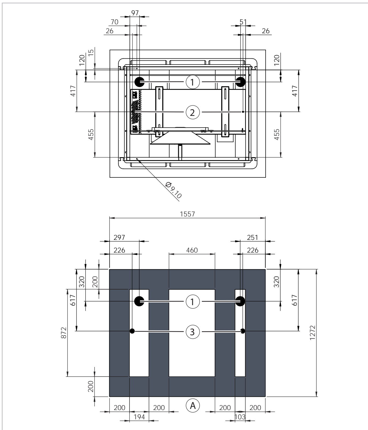
Fig. 8: Strip foundation SWK 4
